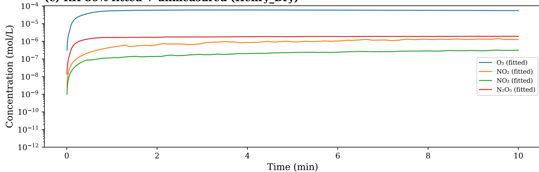
(c) RH 80% fitted + unmeasured (Henry_Dry)
